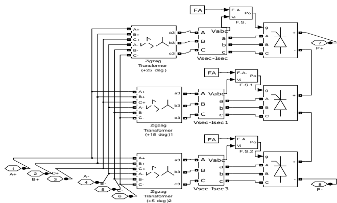
Fig. 7 Thirty six pulse controlled converters with resistive load
