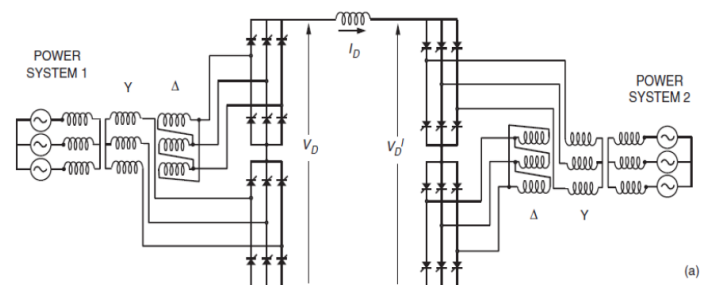
Fig 5: Typical HVDC circuit system
