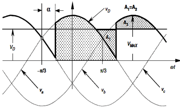
Fig 1: Instantaneous DC voltage V_D , firing angle \alpha and average dc voltage V_D of half wave rectifiers.
