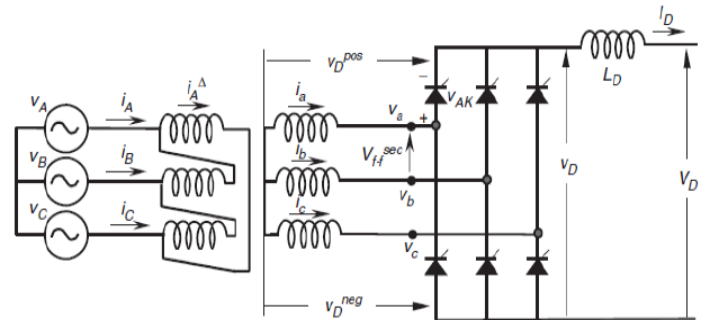
Fig 3: Three-phase full-wave rectifier
