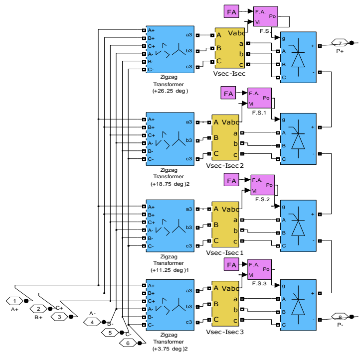
Fig. 8 Thirty six pulse controlled converters with resistive load
