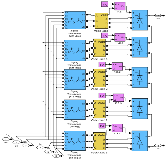
Fig. 9 Thirty six pulse controlled converters with resistive load
