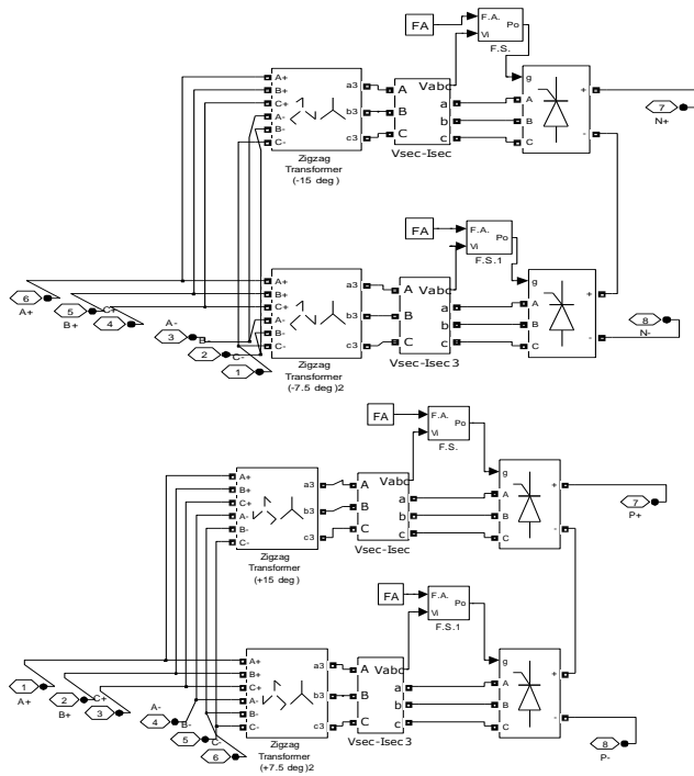
Fig. 6 Twenty Four pulse controlled converters with resistive load
