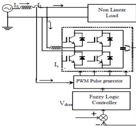
Figure: 4 Fuzzy controlled improved power quality converter
