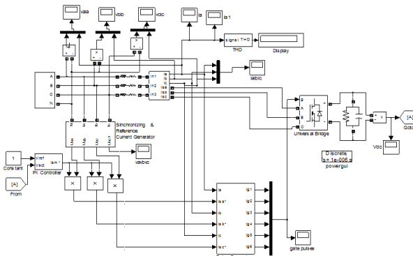
Figure: 6 simulated power circuits for PI controlled improved power quality converter
