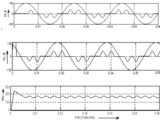
Figure: 8 Waveform without controller
