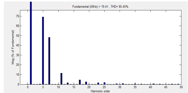
Figure: 10 Harmonics spectrum with PI controller
