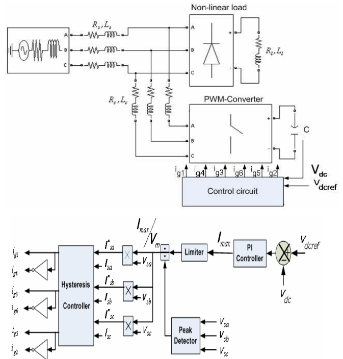
Figure: 2 (a) Active filter system, (b) Active filter system using PI controller
