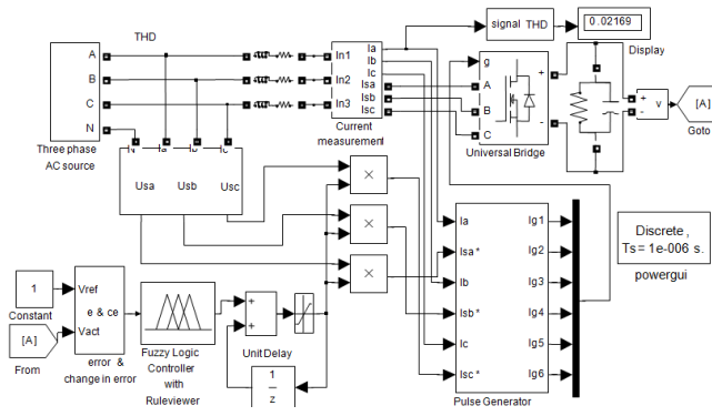
Figure: 7 simulated power circuit for Fuzzy controlled improved power quality converter
