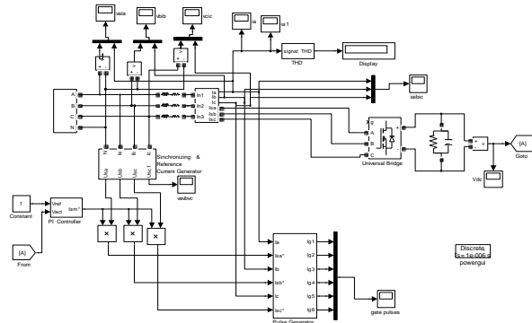
Figure: 5 simulated power circuit without controlled improved power quality converter
