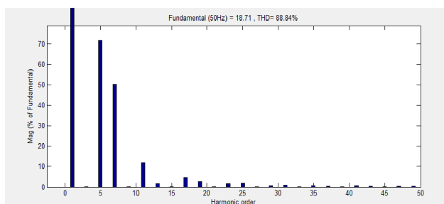
Figure: 9 Harmonics spectrum without controller
