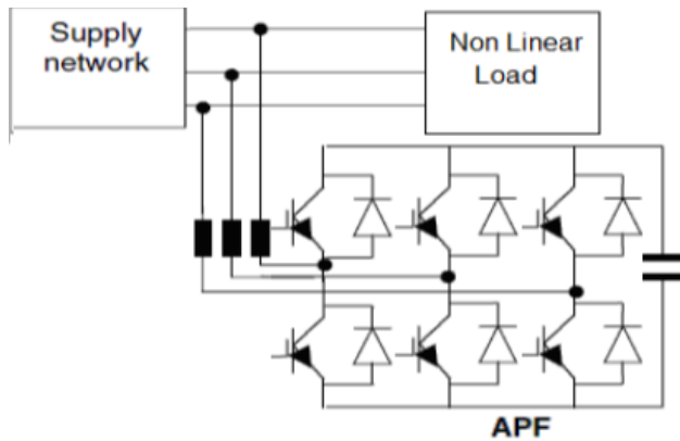
Figure: 1 Active power filter with transmission line
