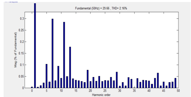
Figure: 11 Harmonics spectrum with Fuzzy controller
