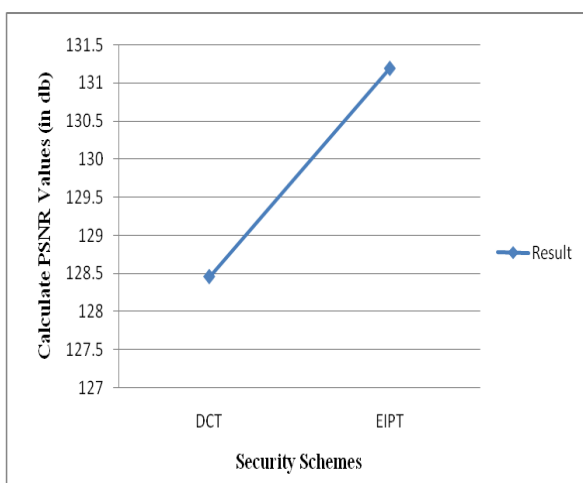
Figure 2 PSNR Based Analysis among Proposed Algorithm and Existing Algorithm
